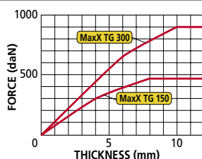
Performance curves with changing load thickness (plate)
